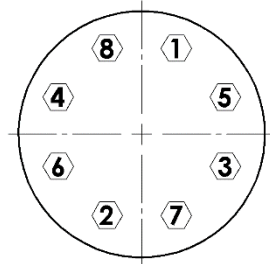
8 BOULONS 8 BOLTS
