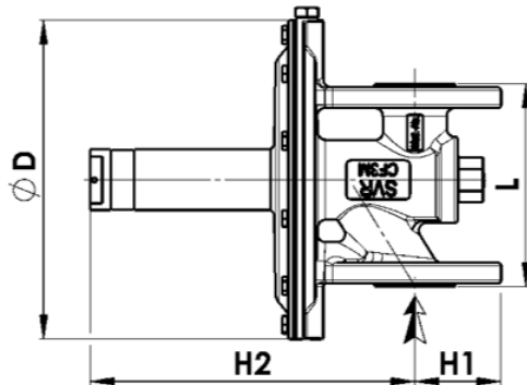
In line excess pressure valve EPL D
