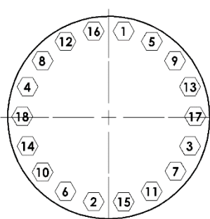
18 BOULONS 18 BOLTS
