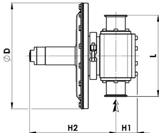
In line clean excess pressure valve Clamp / Threaded EPL D CL
