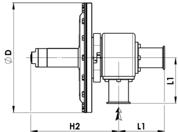
Angle clean excess pressure valve Clamp / Threaded EPL L CL
