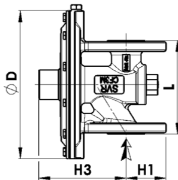
In line air-cushion excess pressure valve EPLCA D
