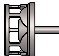
CLAPET A FENETRES WINDOWS PLUG
