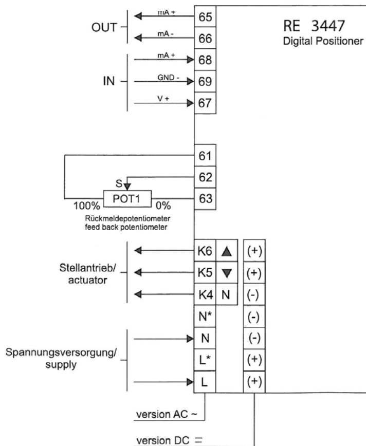
Wiring diagram / Raccordement
